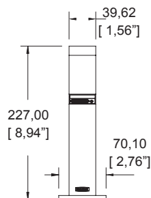
VISTA FRONTAL
