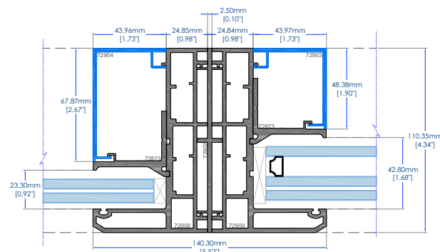
MULLION
