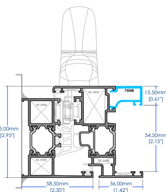
SWING IN WINDOW SYSTEM
