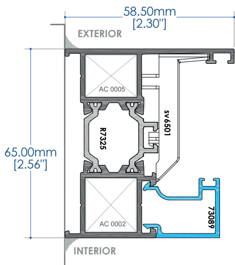
INSULATED
