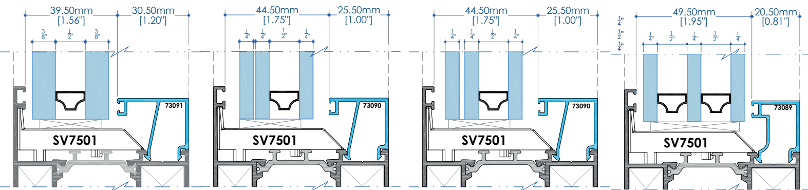
INSULATED
