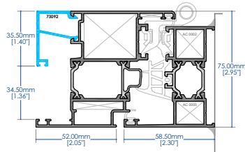
SWING IN DOOR SYSTEM
