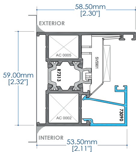
INSULATED
