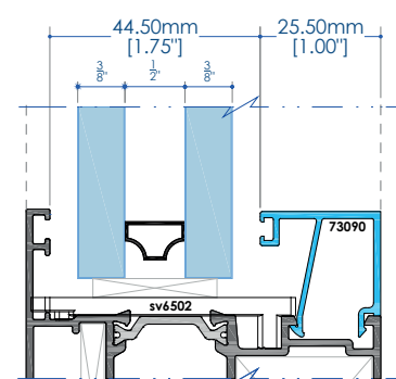
INSULATED
