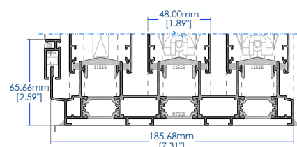
○ 3 track frame with mosquito screen 7.31"
