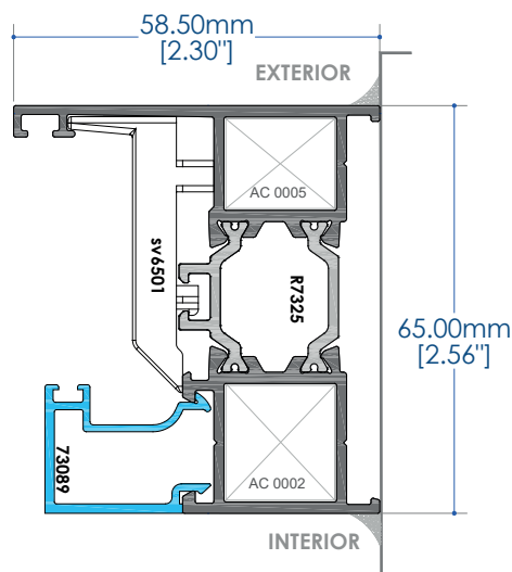
INSULATED
