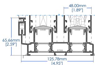
○ 2 track frame with mosquito screen 4.95"
