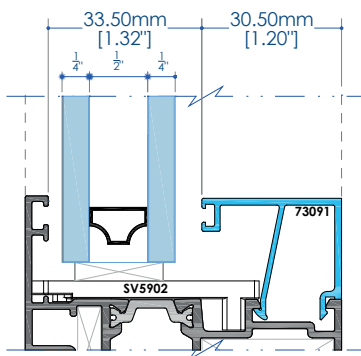
INSULATED
