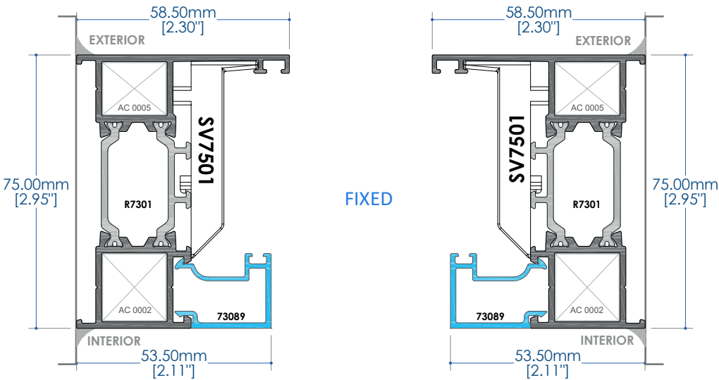
LAMINATED INSULATED
