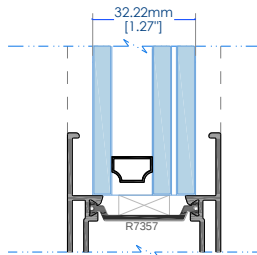
INSULATED LAMINATED
