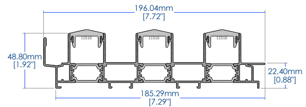
3 track frame
