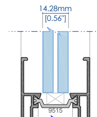
LAMINATED * Special gaskets needed
