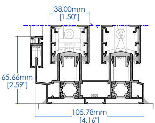
○ 2 track frame with mosquito screen 4.16"
