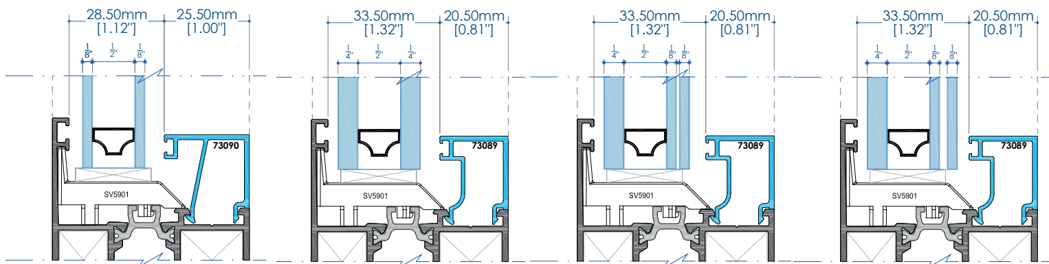
INSULATED
