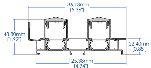
2 track frame
