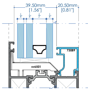
LAMINATED INSULATED
