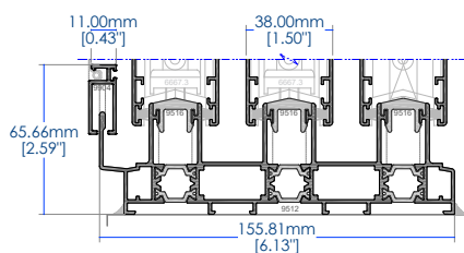
○ 3 track frame with mosquito screen 6.13"
