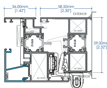
SWING IN WINDOW SYSTEM
