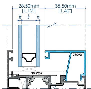
INSULATED
