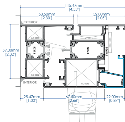
SWING IN DOOR SYSTEM
