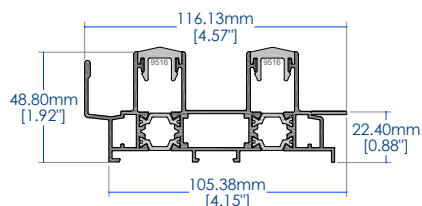
2 track frame
