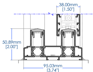
○ 2 track frame 3.74"
