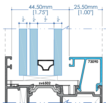
LAMINATED INSULATED
