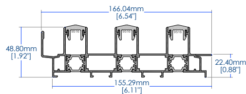
3 track frame
