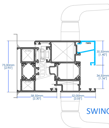
INSULATED
