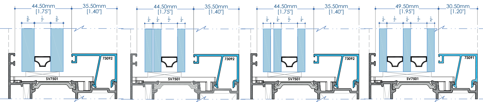
INSULATED
