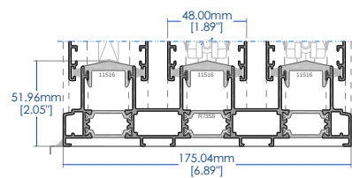
○ 3 track frame 6.89"
