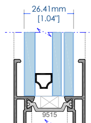
INSULATED LAMINATED
