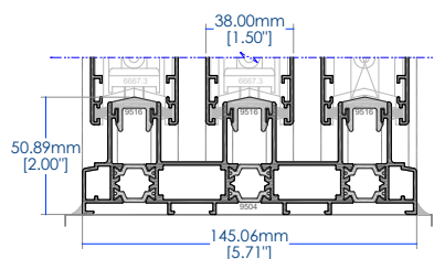
○ 3 track frame 5.71"
