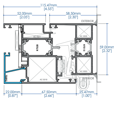
SWING IN DOOR SYSTEM
