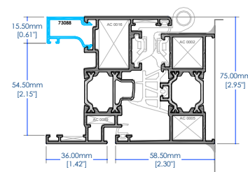
SWING IN WINDOW SYSTEM
