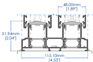
○ 2 track frame 4.53"
