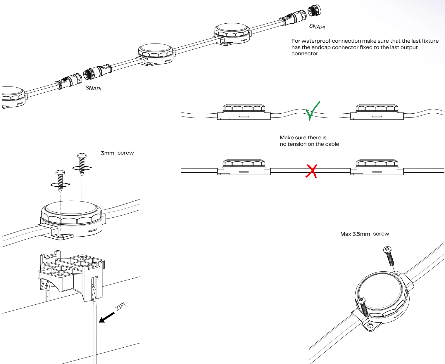
Tube clip fixation
